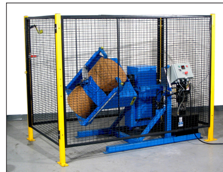
Tilt-To-Load Drum Tumbler with Automated Control Package and Safety Enclosure
