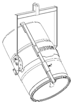
Figure 2.2 Kit # 4556-P Bracket Assembly RIMLESS plastic drum shown being lifted with Kit # 4556-P Bracket Assembly installed.
