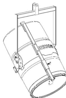
Figure 2.3 4560-P Top Rim Clamp Assembly RIMMED plastic drum shown being lifted with Kit # 4560-P Top Rim Clamp Assembly installed.
