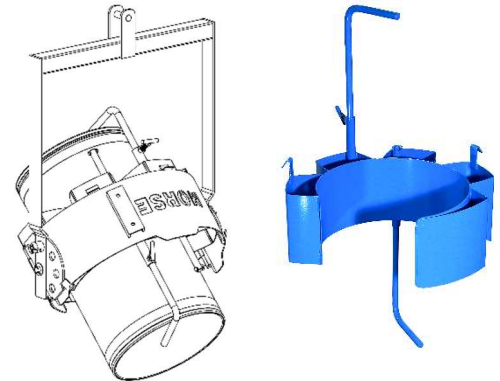
Figure 2.1 55/30 Series Diameter Adaptors Model 85i shown with Diameter Adaptor # 55/30-16 for 15.5" to 16" diameter drum
