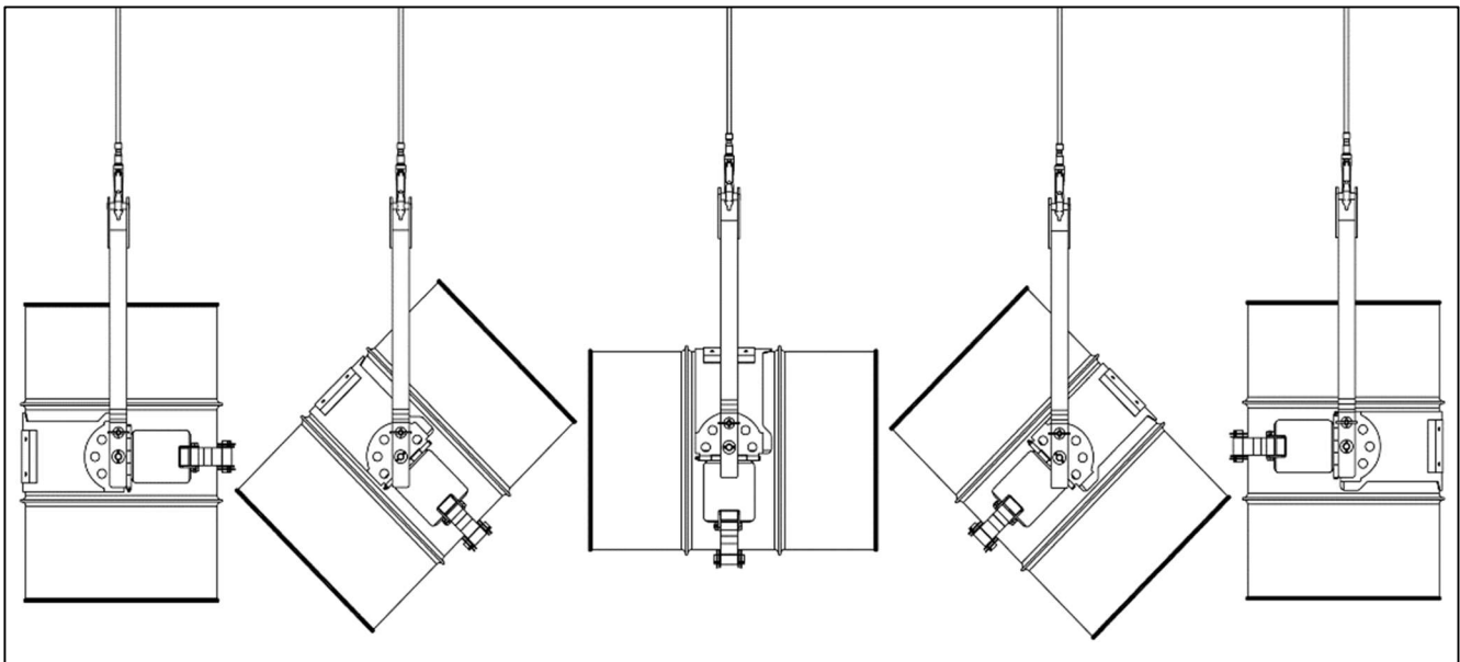
Model 85i Tilt Lock Positions
