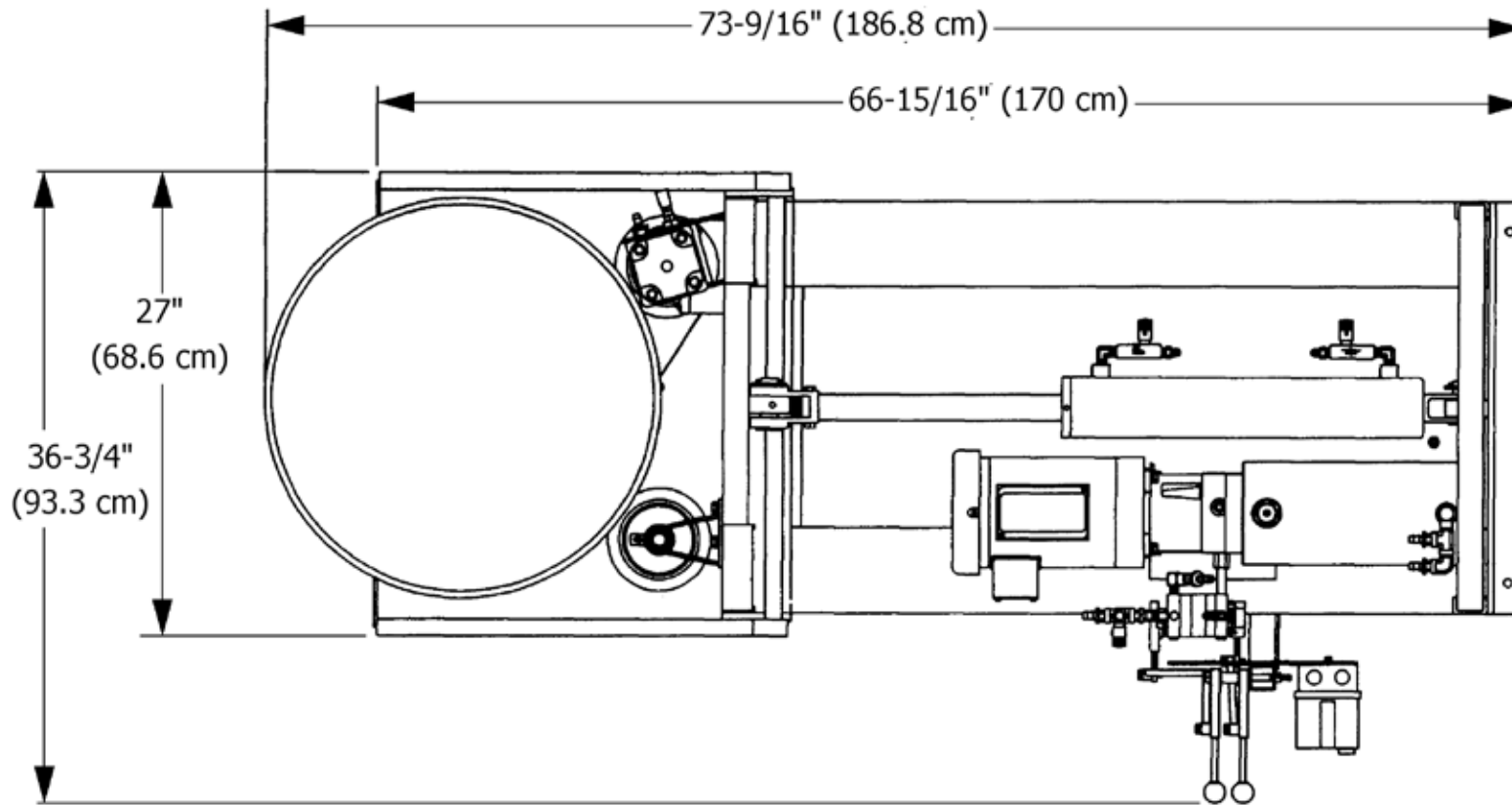
TOP VIEW LOADING POSITION
