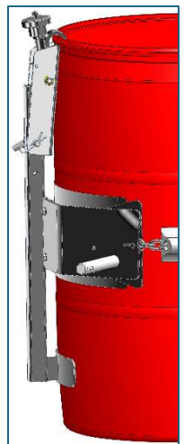
Figure 2.2 Stainless Steel Kit # 4560BSS-P Install Top Rim Clamp Kit to handle RIMMED plastic drum
