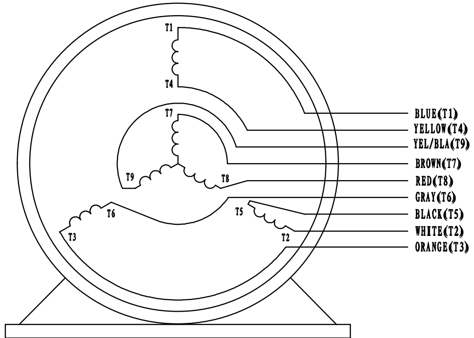
VIEW OF TERMINAL END
