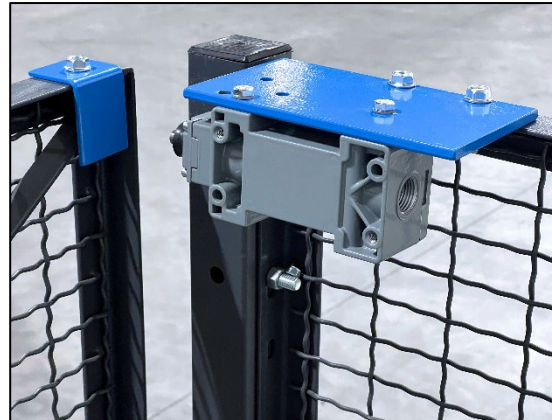
Morse Switch Assembly (Kit 3597KIT-P) installed at enclosure gate opening
