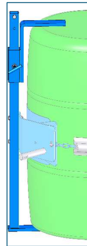
Figure 2.1 Kit # 4556-P Install Bracket Assembly Kit to handle RIMLESS or RIMMED plastic drum
