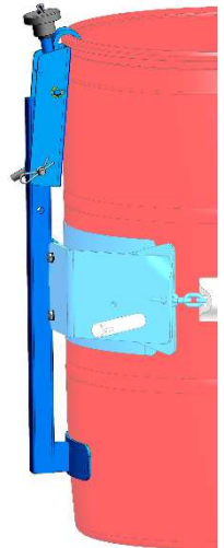
Figure 2.2 Kit # 4560B-P Install Top Rim Clamp Kit to handle RIMMED plastic drum
