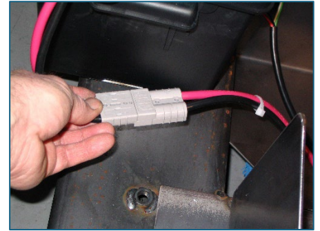
13. Plug battery to pump. Test unit function for forward and reverse.
