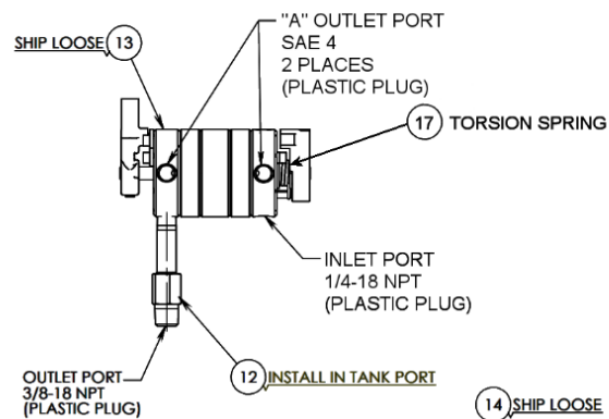
SCHEMATIC
