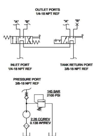
SCHEMATIC
