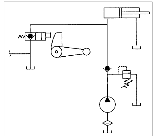
Hydraulic Schematic
