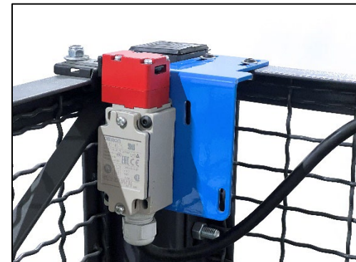
Close enclosure and verify that the key aligns properly with the switch. If key is not aligned properly, adjust accordingly. Key may be adjusted by loosening its screws and moving, then re-tightening screws. Use zip ties to retain cable from switch to control station.
