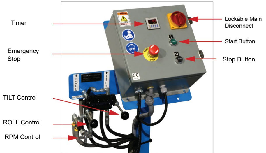
Figure 3.1 Control Station
