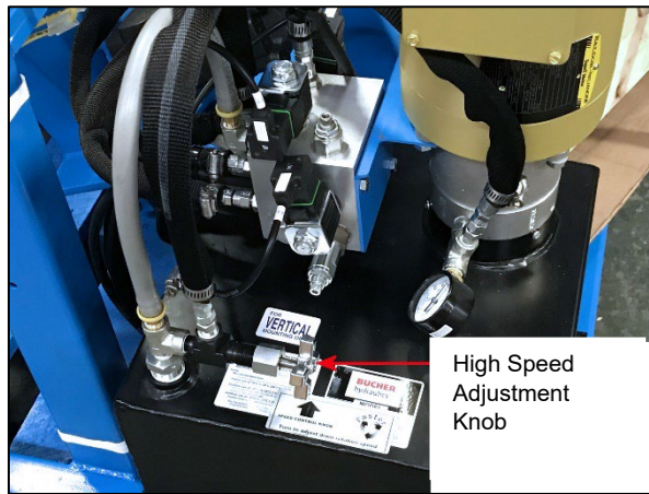
Hydraulic Manifold
