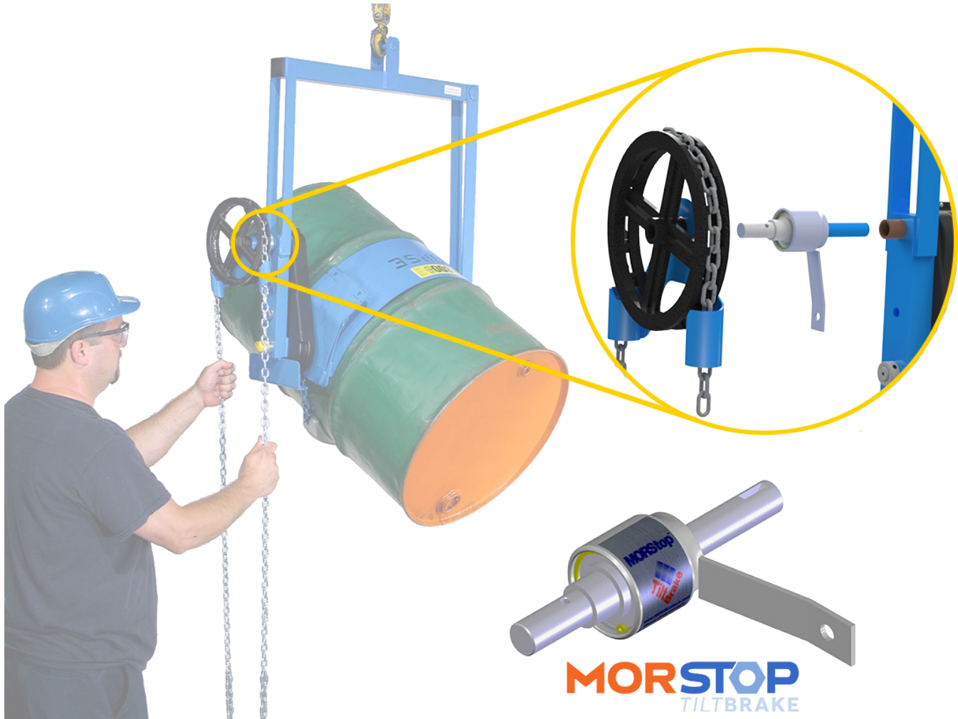
MORStop™ Tilt-Brake on model 185A Kontrol-Karrier
